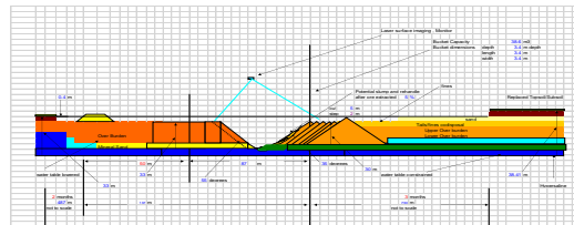
Drag Line Layout for Mineral Sands
